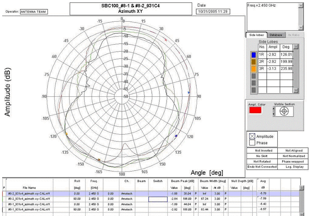
Radiation Pattern
