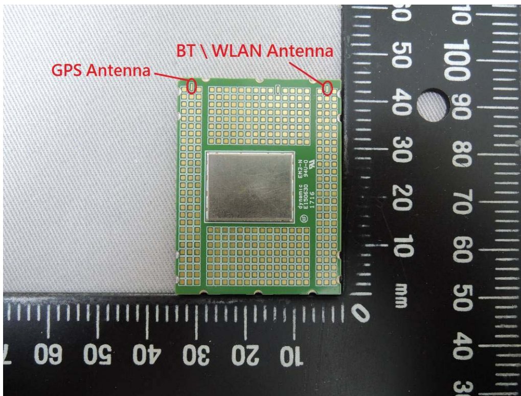
BT/WLAN/GPS Antenna PIN
