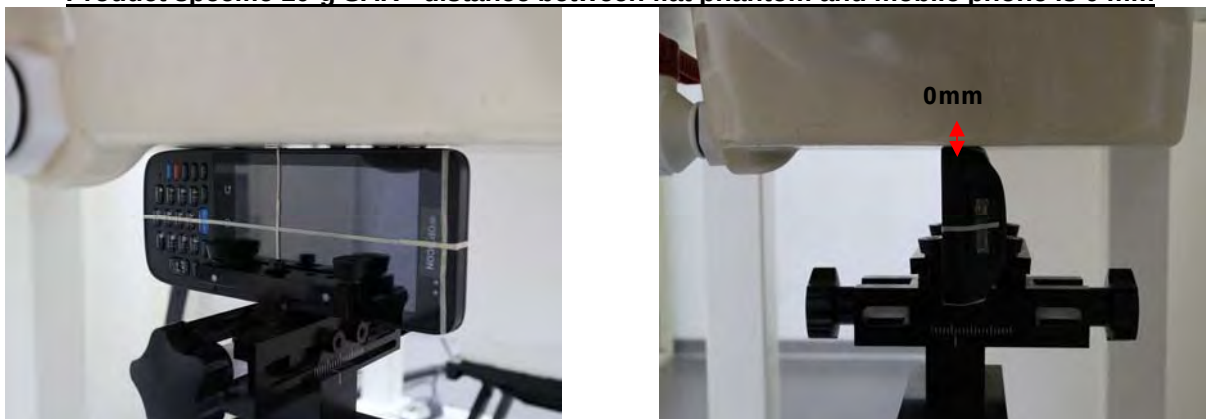
Fig.12 EUT Left side to flat phantom
