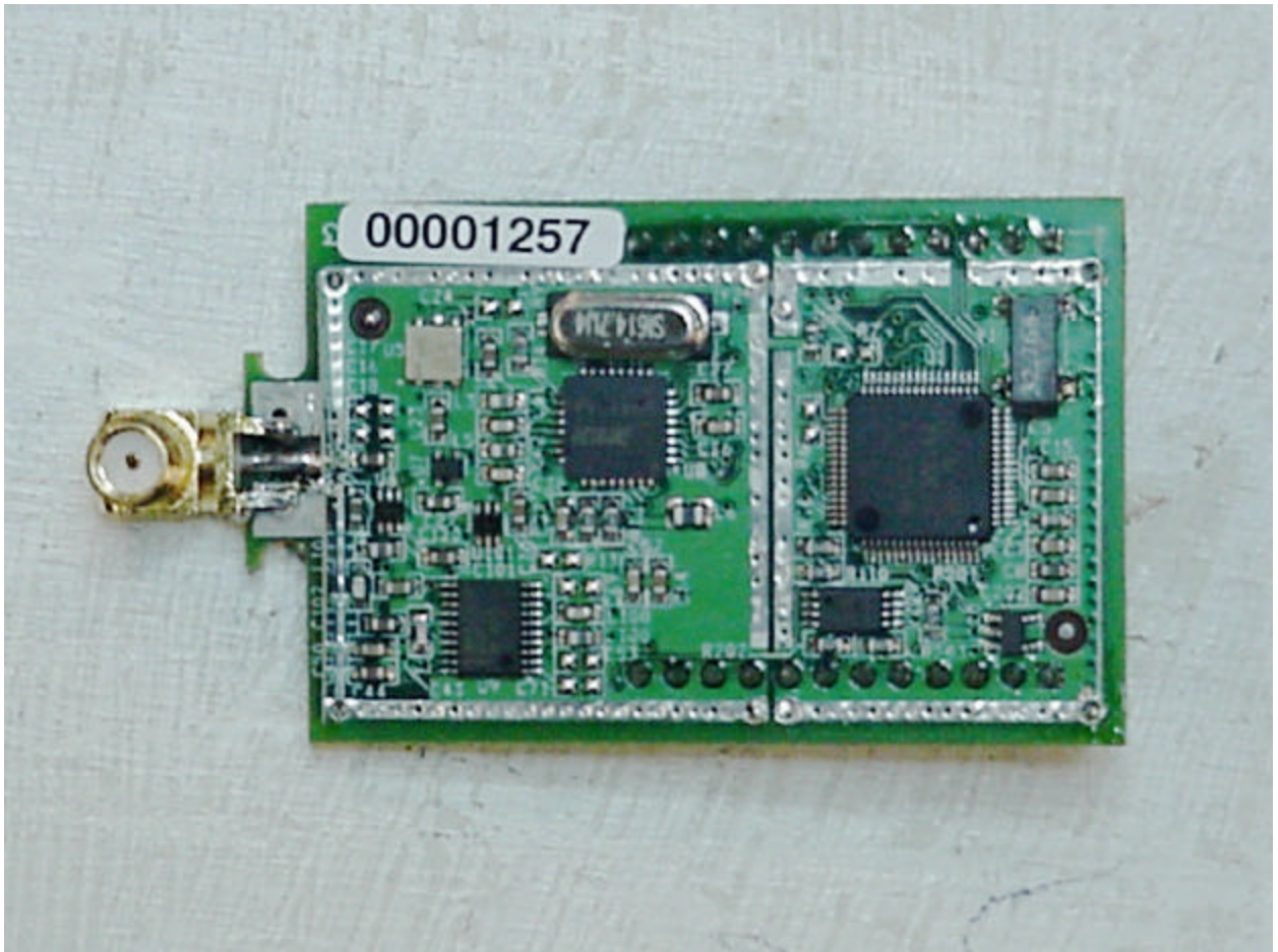
Photo 2. Top View of EUT With Shield Removed
