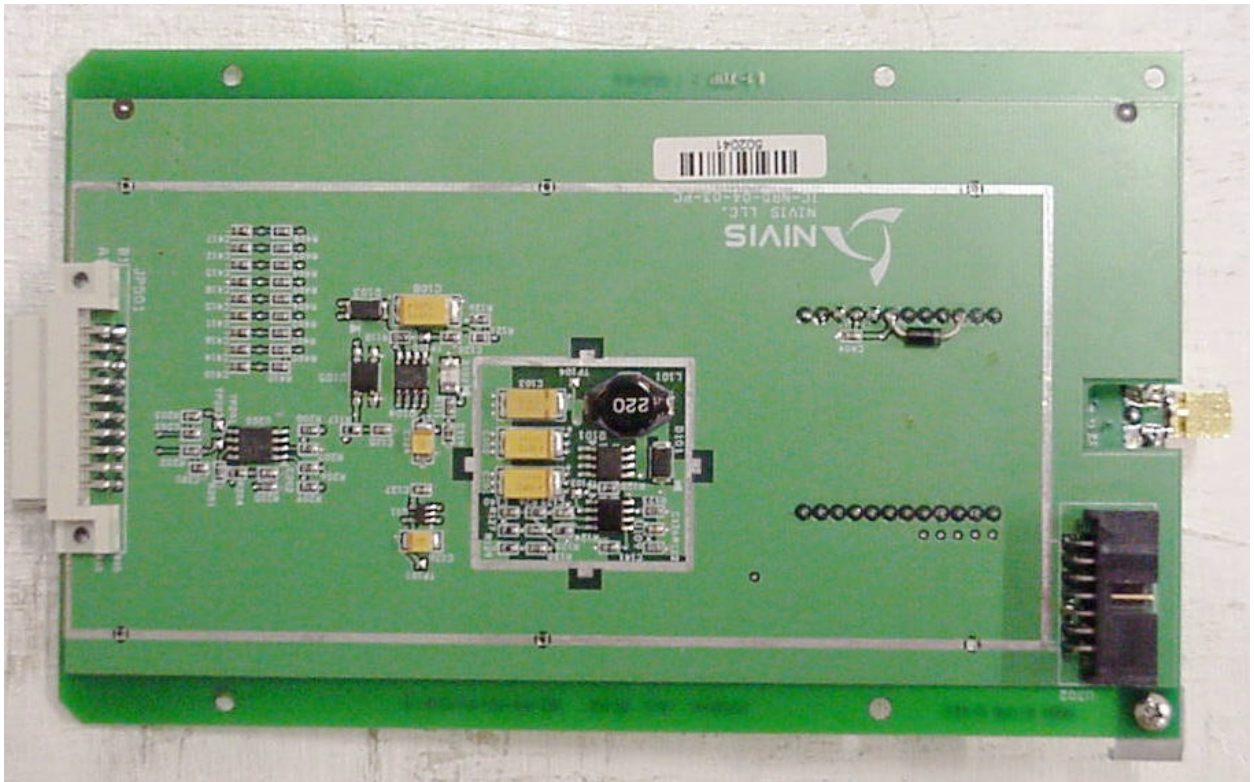
Photo 7. Circuit Side of EUT Mounting PWB
