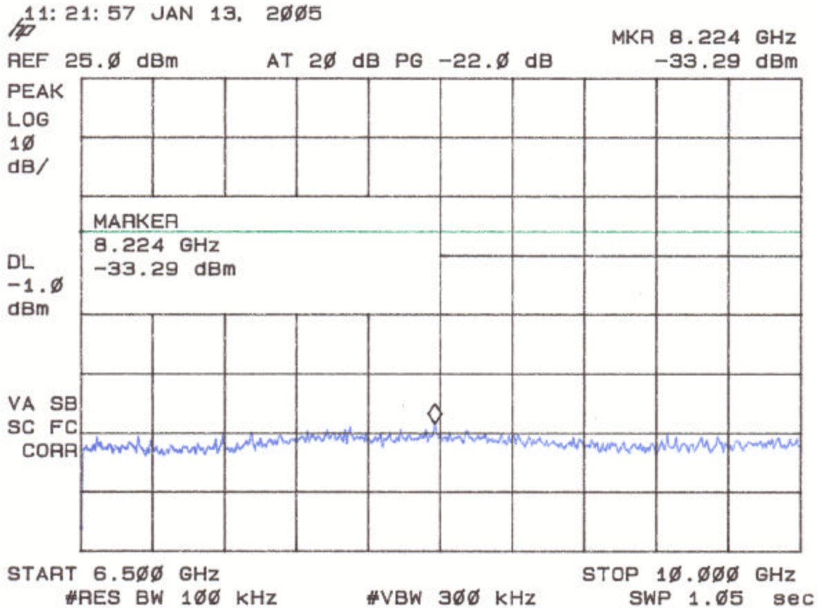
Figure 4l Antenna Conducted Spurious Emissions 15.247(c) (High Channel) Dual Band Antenna
