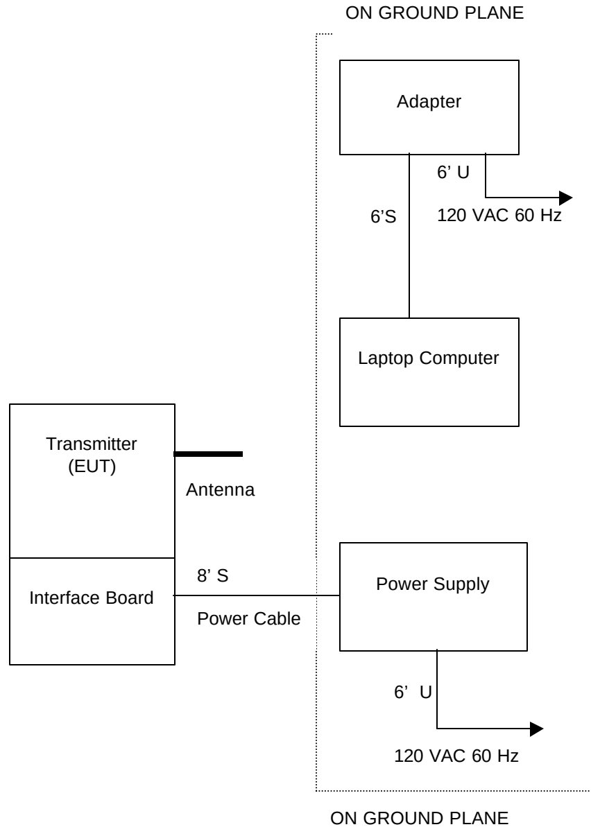
FIGURE 1 TEST CONFIGURATION
