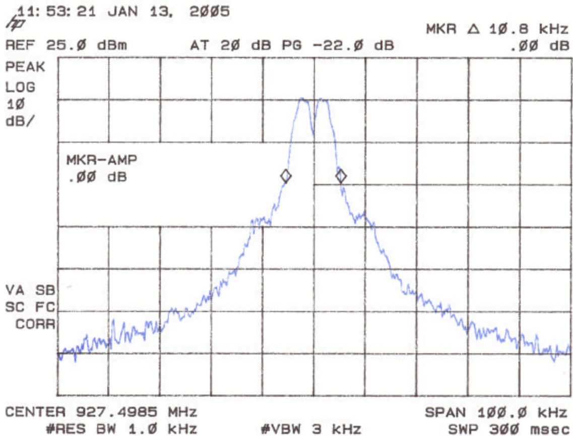
Figure 6c. 20 dB Bandwidth per FCC Section 15.247(a)(1)(ii) (High Channel) Dual Band Antenna
