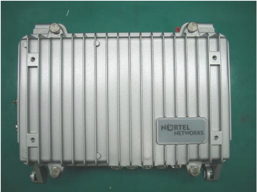
Front view of the APU
