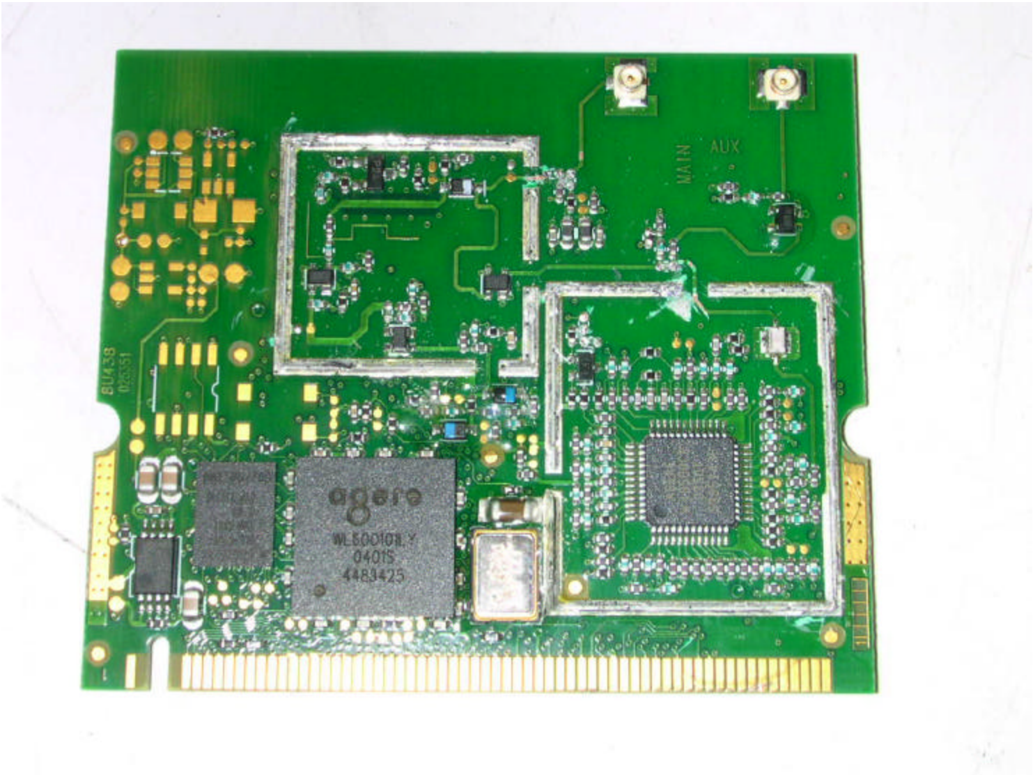
WLAN Radio PCB (with shield covers removed)
