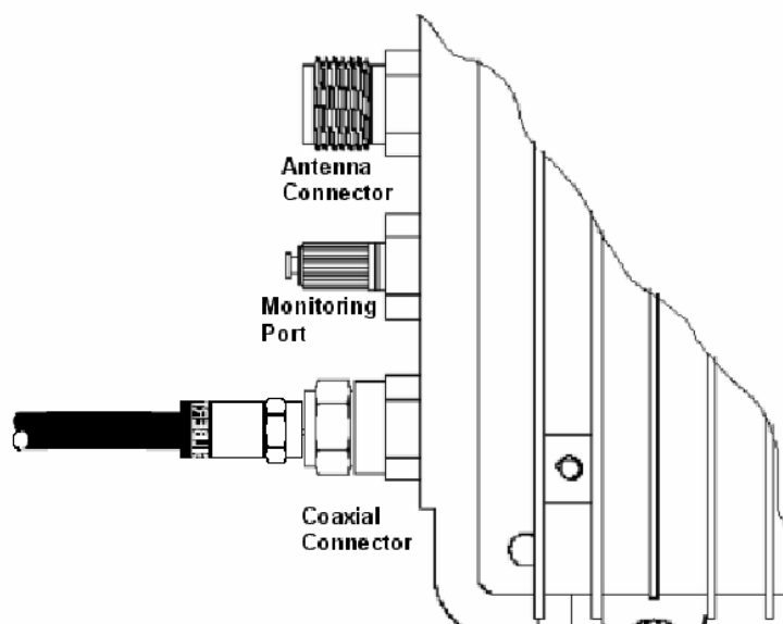
Figure 3-21 Connecting the coaxial cable to the connector port
