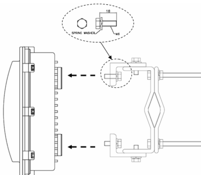
Figure 3-26 Assembling the mounting bracket on the CSU
