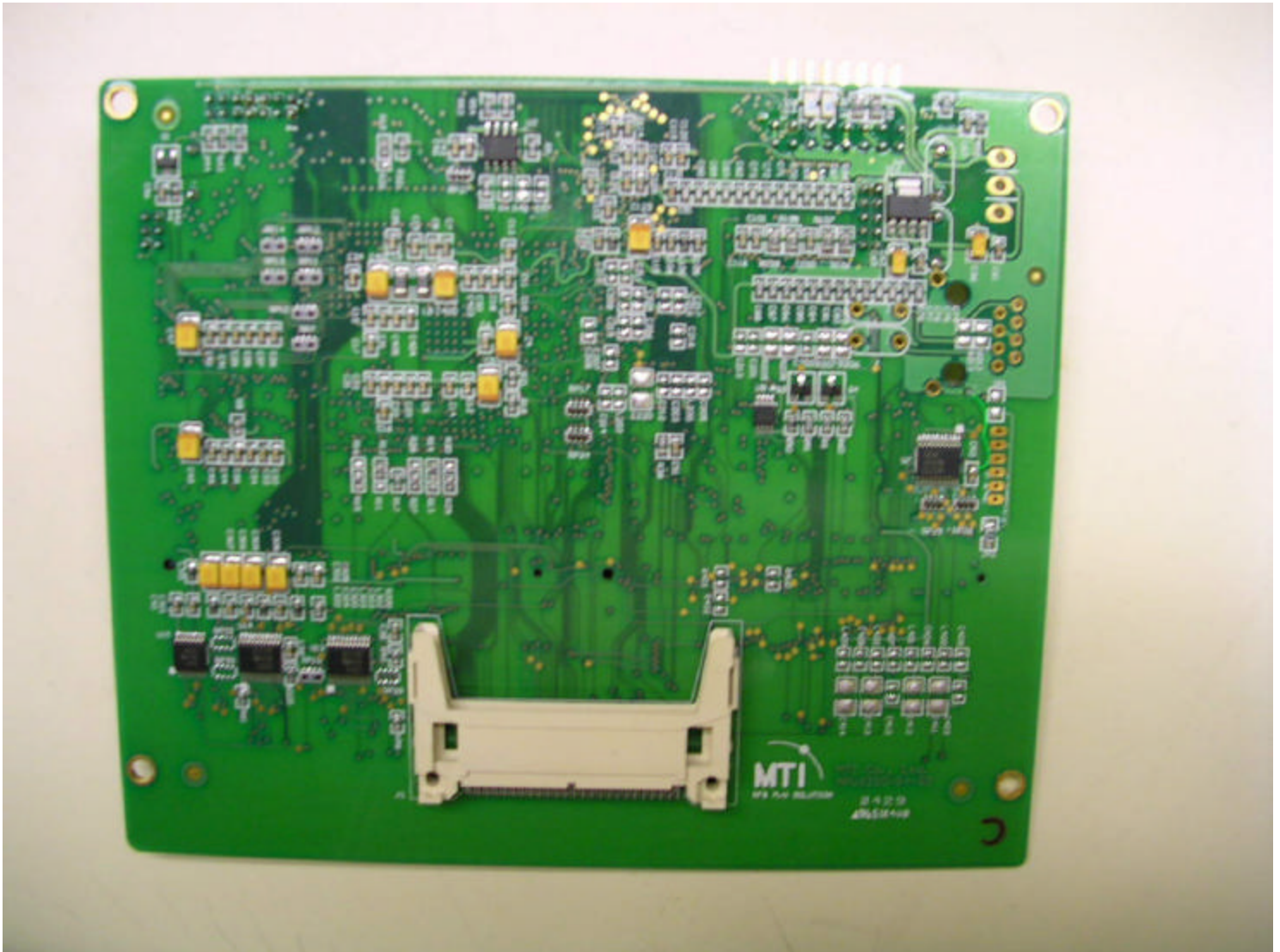
Secondary side of Access Point board
