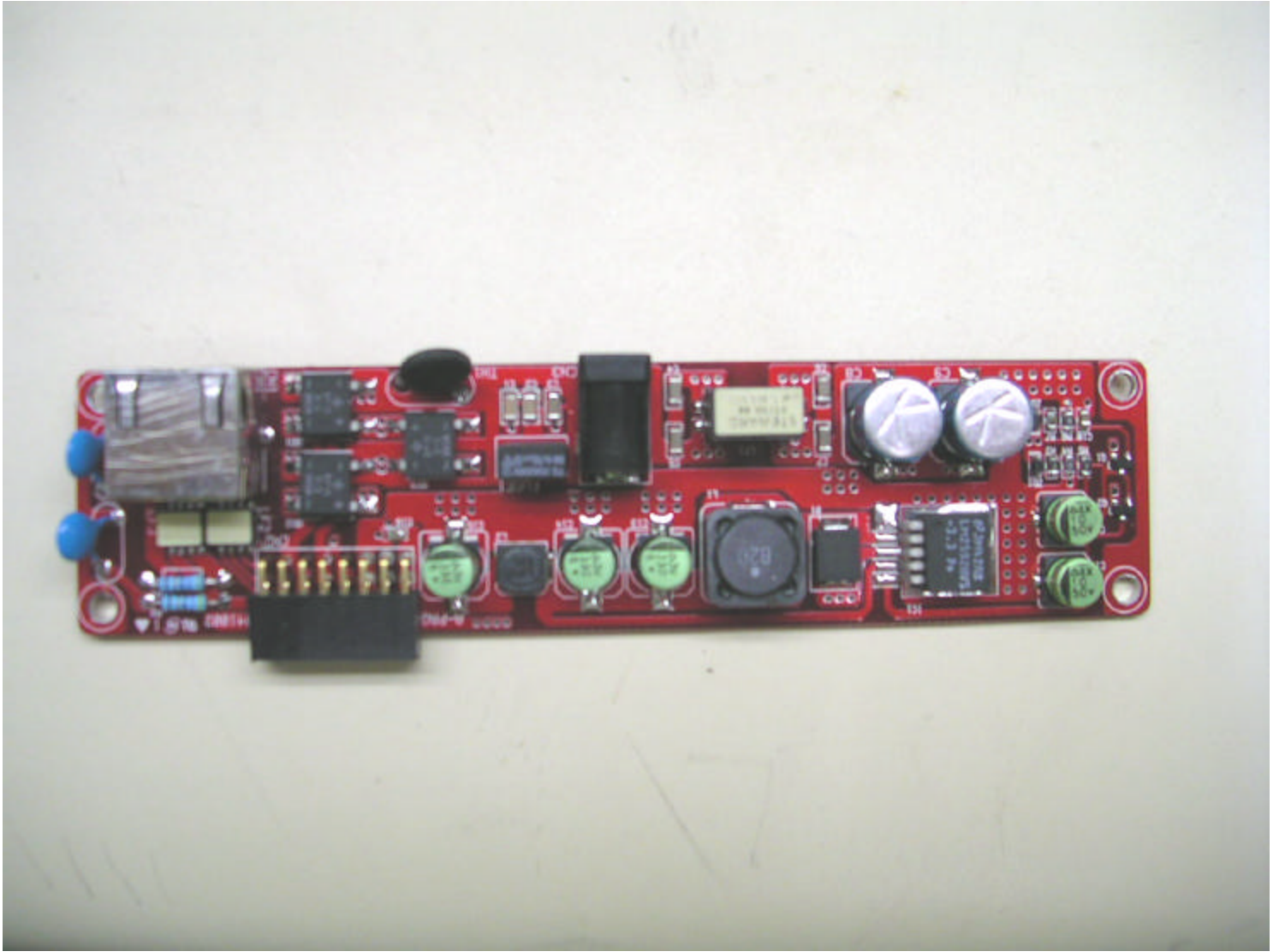
Component side of power supply board
