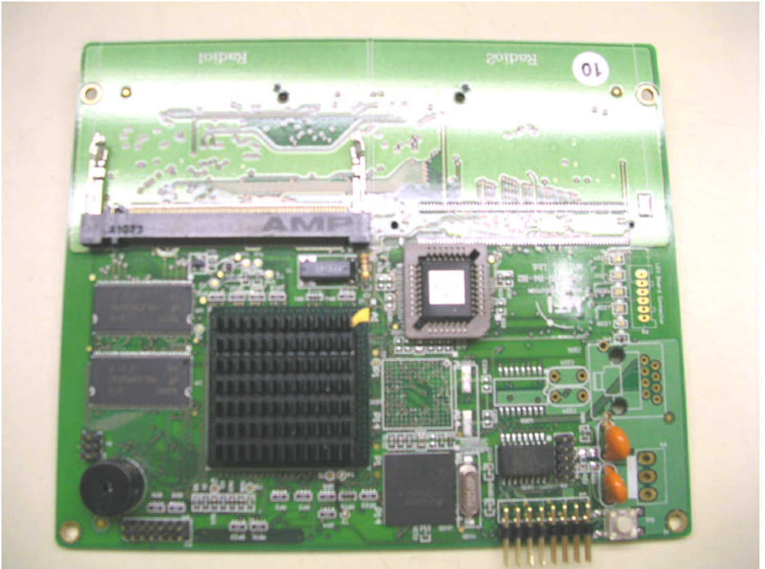
Component side of Access Point PCB
