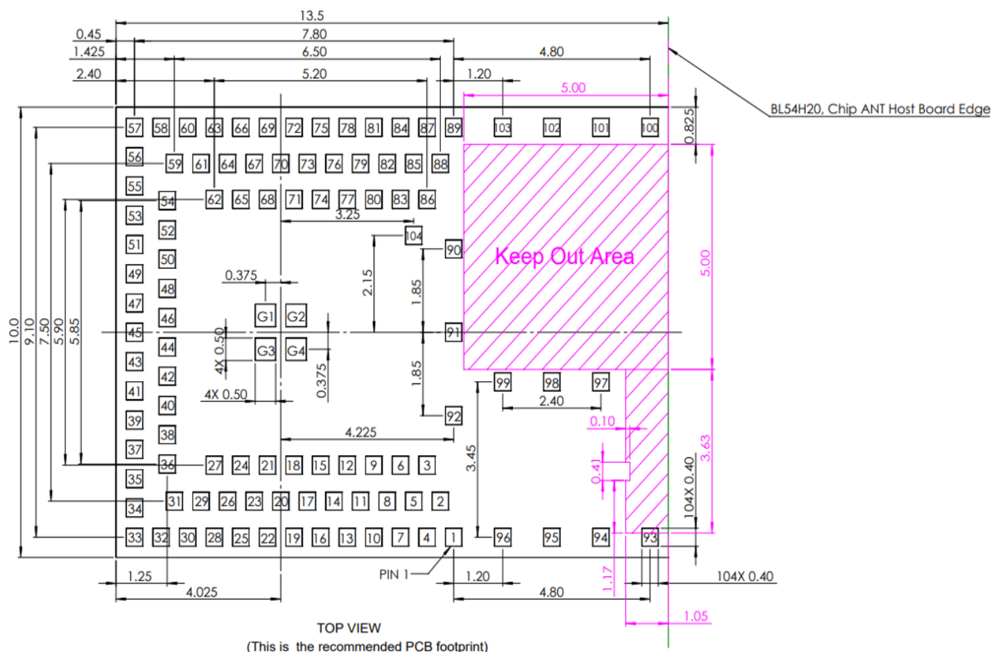
Figure 11: Land pattern 453-00xxx and Keep-out for the 453-00197
