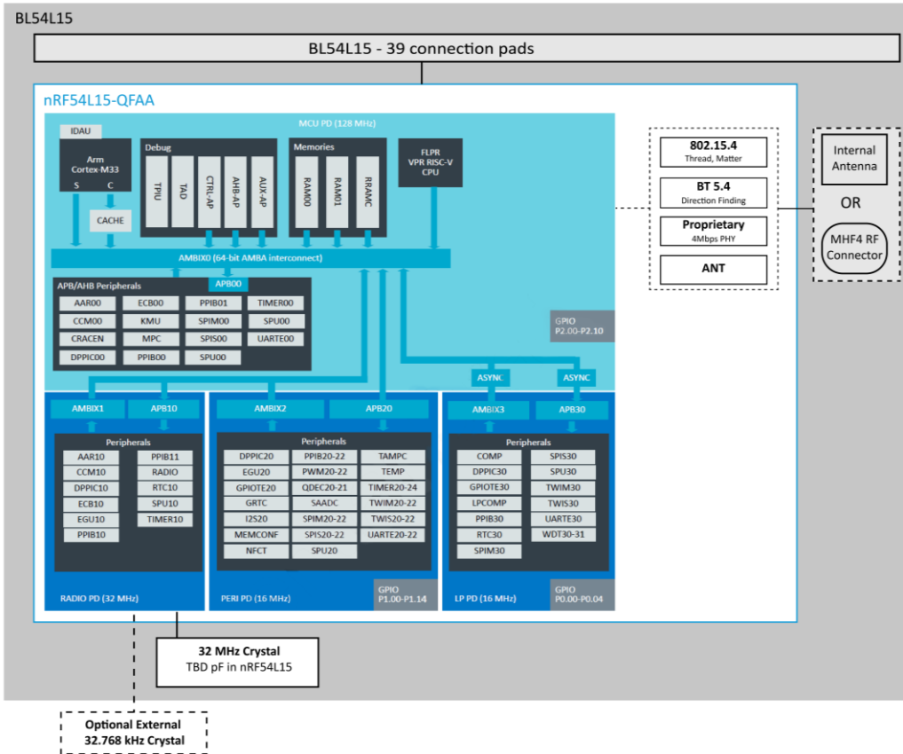
Figure 1: BL54L15 HW block diagram
