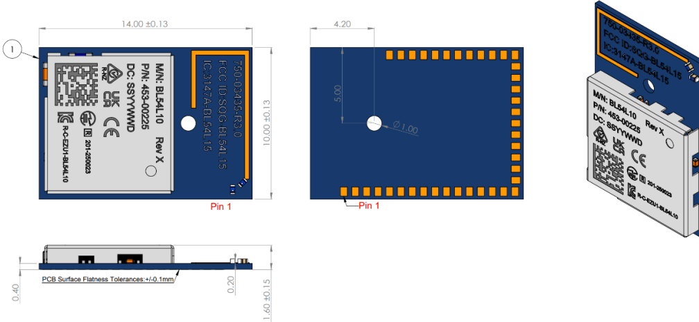
Figure 8 : Mechanical Details – Internal Antenna variant module (453-00225)
