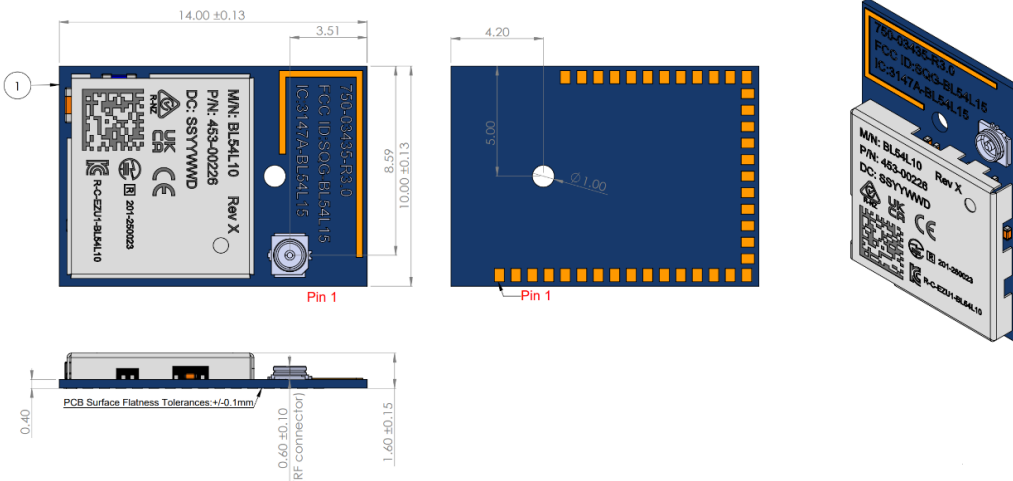
Figure 10 : Mechanical Details – MHF4 RF connector variant module (453-00226)
