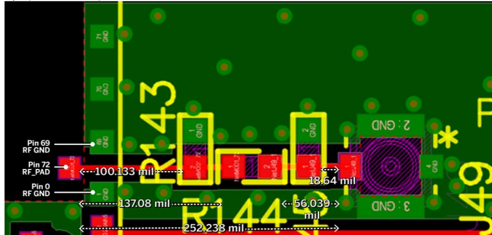
Layer1 (RF Track and RF GND)
