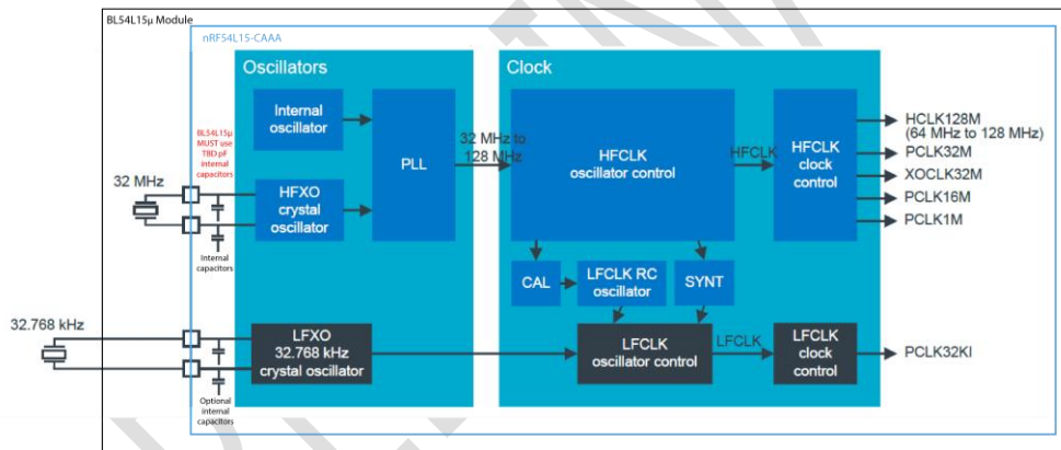
Figure 4: nRF54L15 Clock System Overview (adapted from Nordic)
