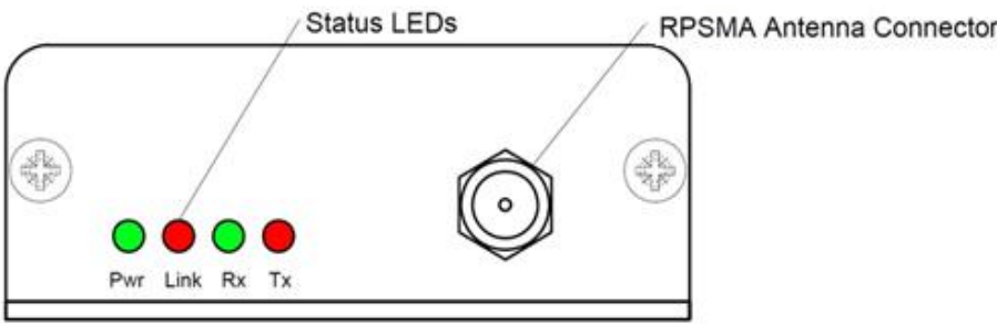
Figure 1: CL4490 Status LEDs
