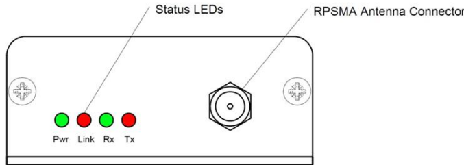
Figure 1: CL4790 Status LEDs
