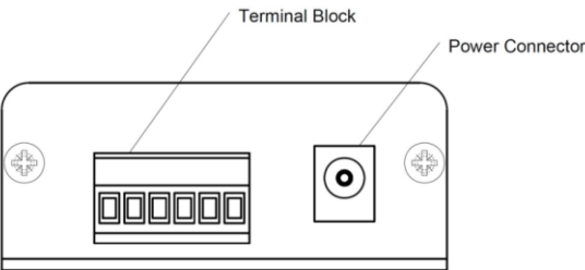
Figure 5: CL4790-RS485
