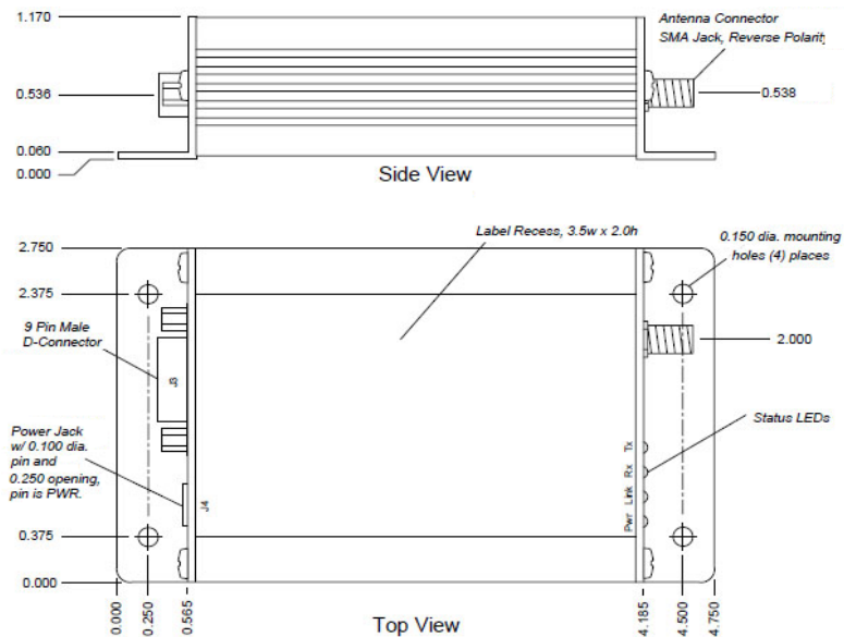
Figure 7: Mechanical Drawing
