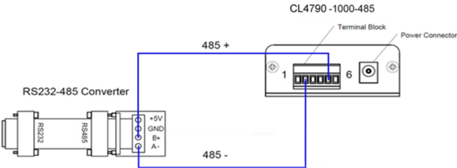
Figure 6: RS232-485 Converter
