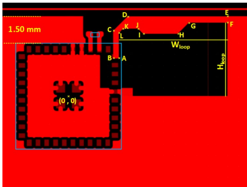
Figure 2: Antenna Layout With Coordinates
