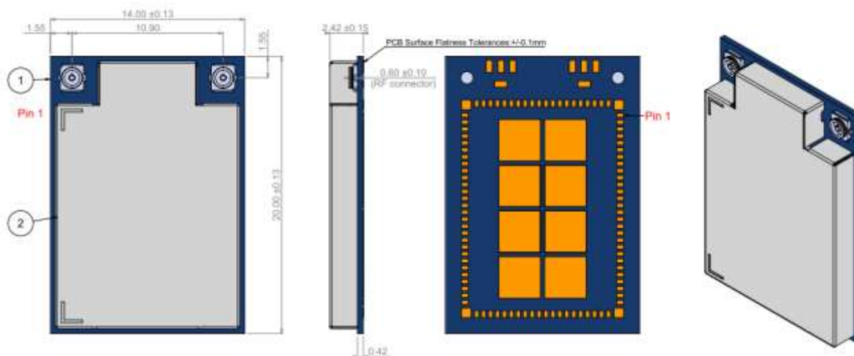
Mechanical dimensions for the Sona MT320 M.2 1420 module.
