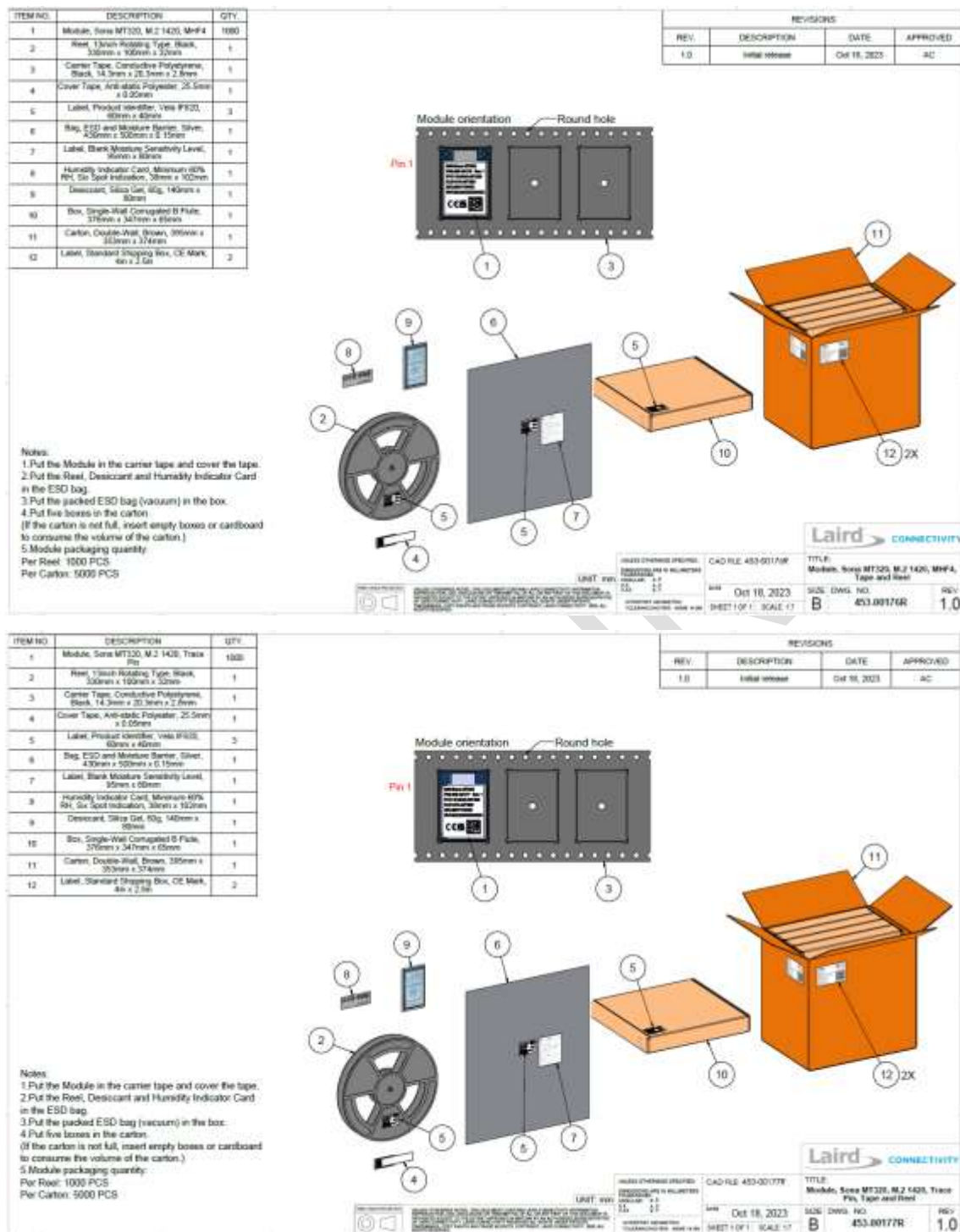
Figure 7: Sona MT320 M.2 1420 packaging processes
