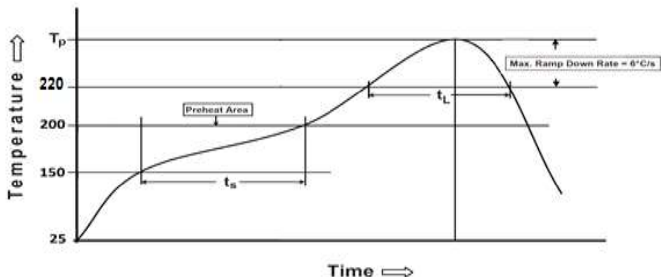
Figure 23: Temperature profile
