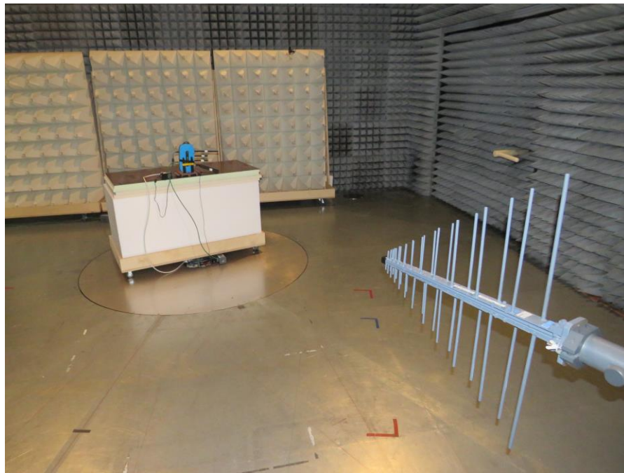
TEST SETUP 200MHz – 1GHz
