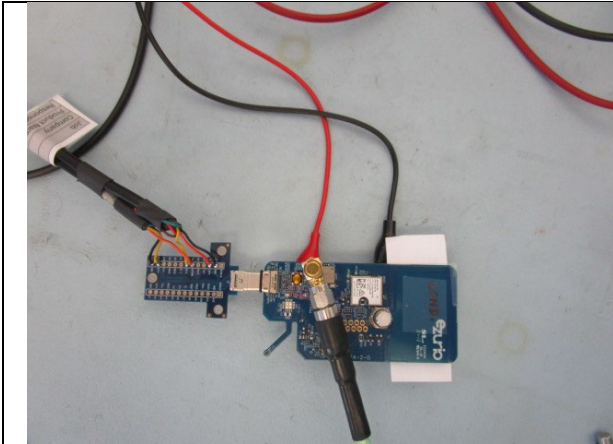
RF Conducted – BLE
