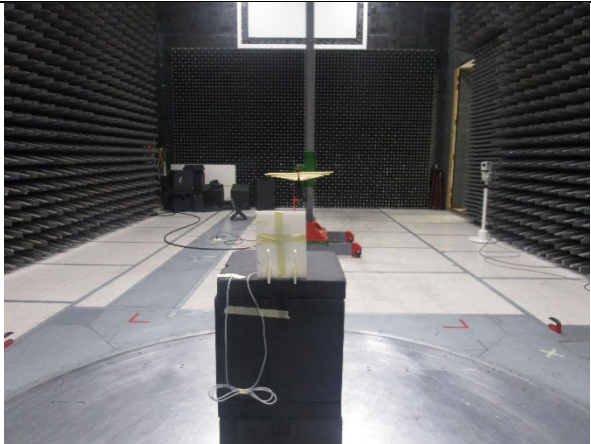
200-1000 MHz (External Sensor)
