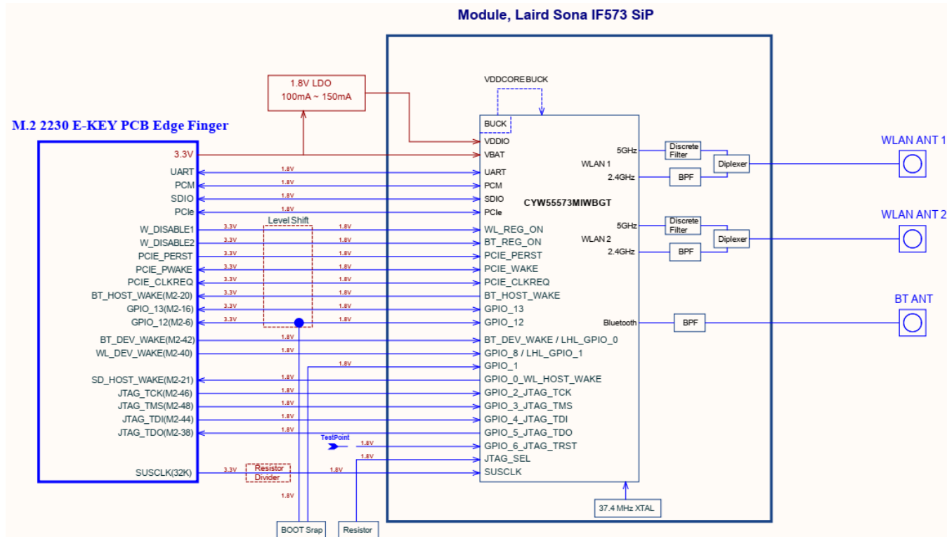
Figure 2: M.2 2230 E-Key
