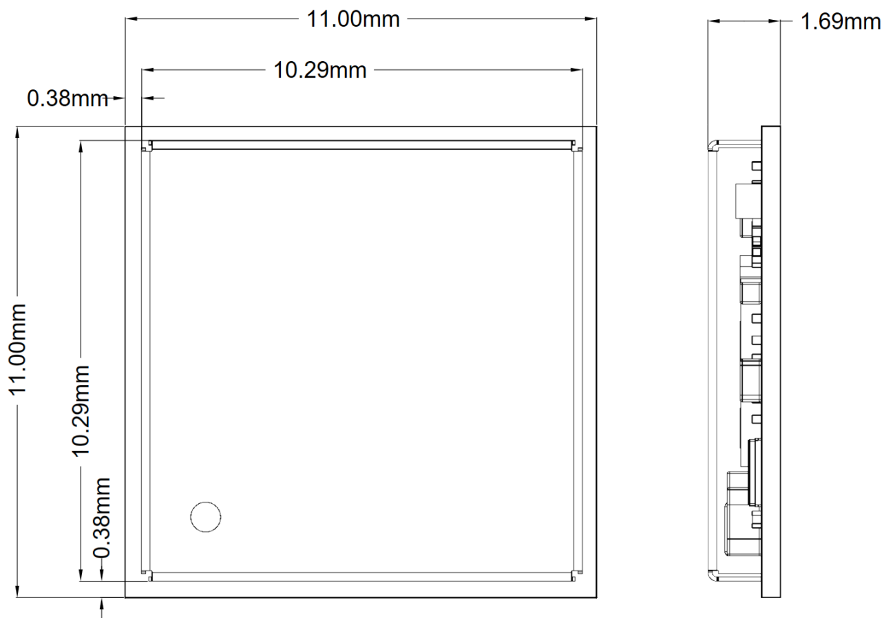
Figure 5: Mechanical Drawing – NX611 SIP module
