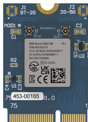
Figure 3: Sona NX611 M.2 2230 Module
