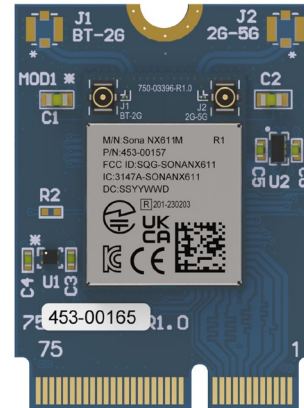
Figure 3: Sona NX611 M.2 2230 Module
