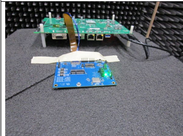
Chip antenna unit
