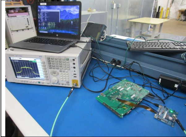
RF Conducted
