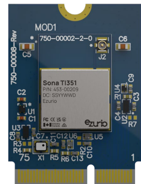
Figure 3: Sona TI351 M.2 2230 Module
