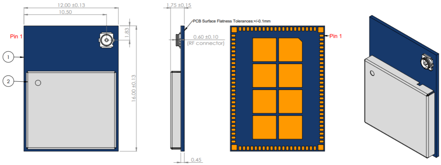
Figure 5: 453-00199 Mechanical Drawing
