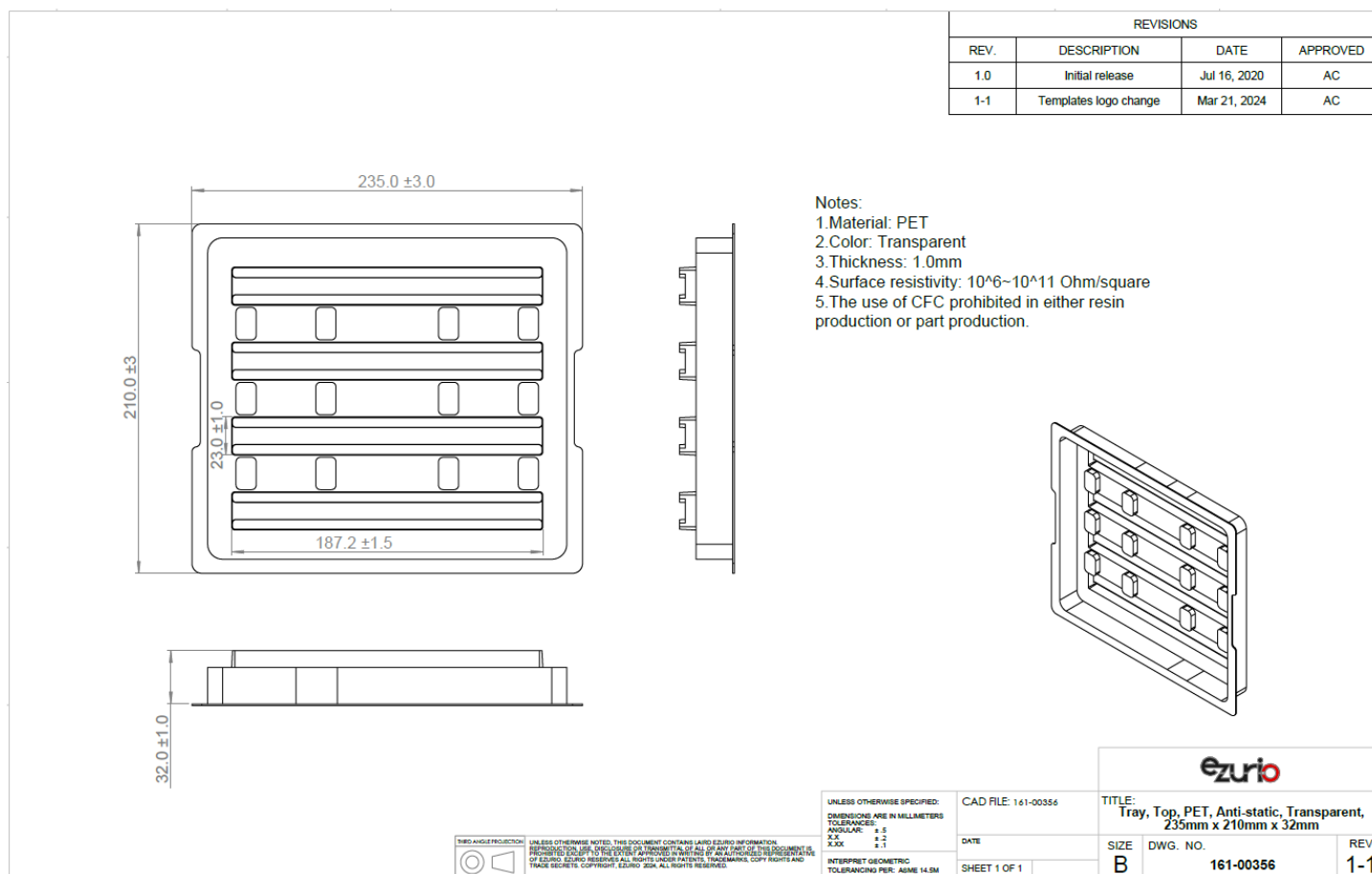
Figure 19: Sona TI351 M.2 2230 Shipping Tray, Top, 161-00356
