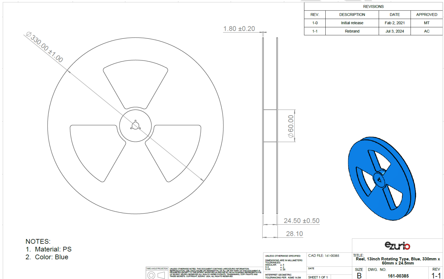
Figure 14: Sona TI351 Reel specifications, 161-00385
