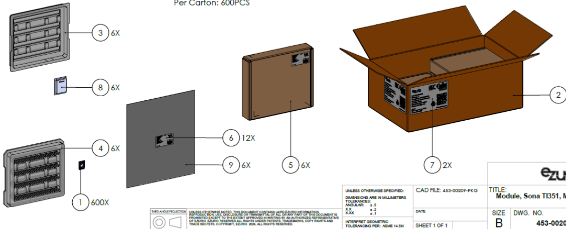
Figure 20: Sona TI351 M.2 2230 Packaging Process, 453-00209-PKG
