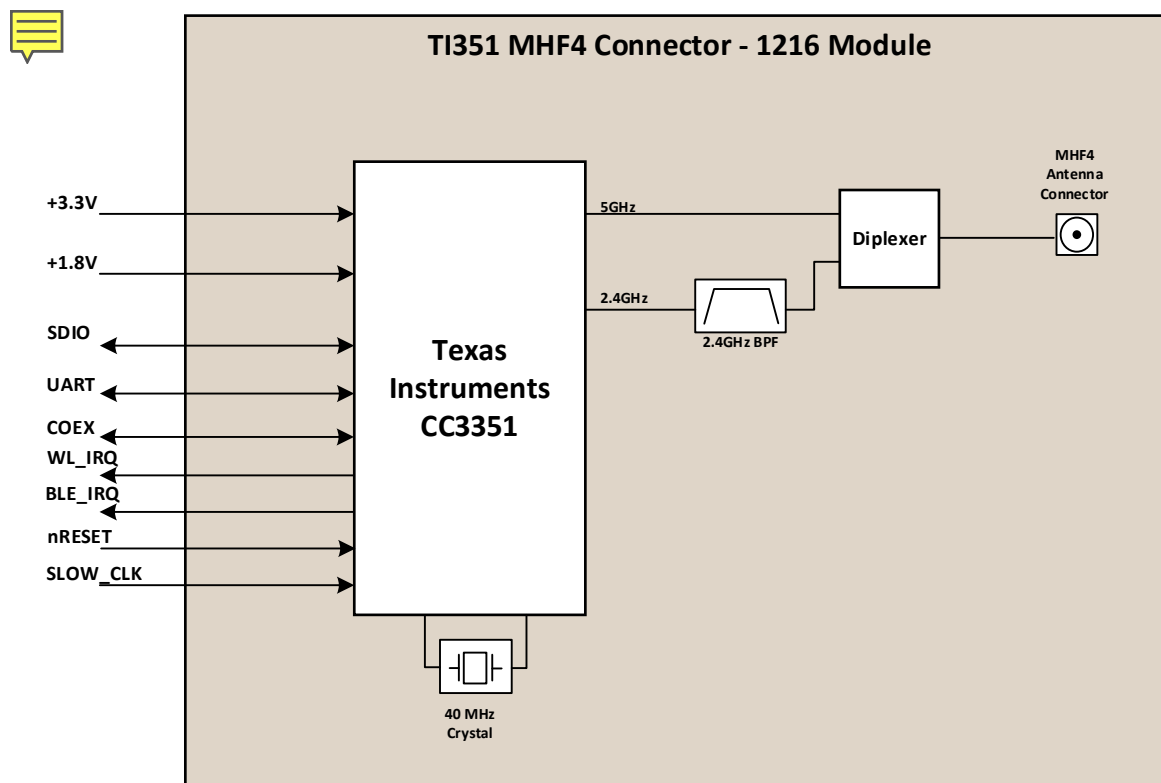
Figure 1: M.2 1216 MHF4L connector variant (453-00199) block diagram
