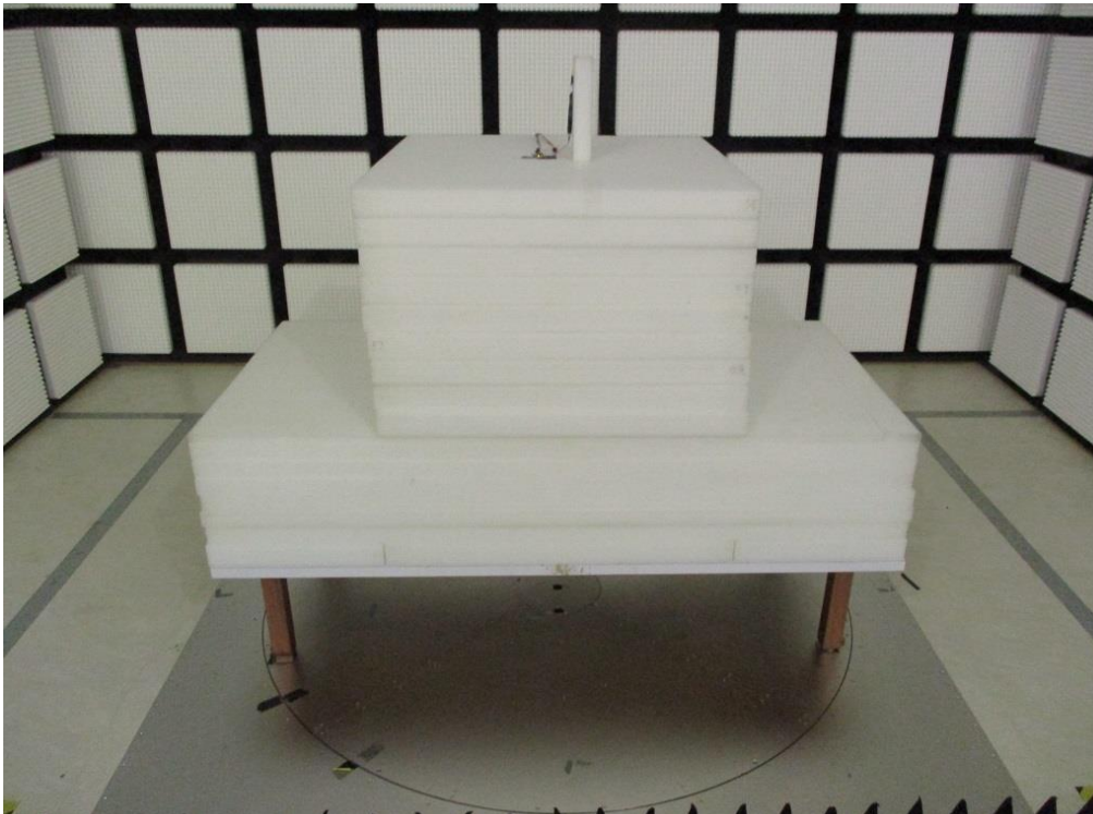
Radiated Emission above Test (Test Configuration 4)
