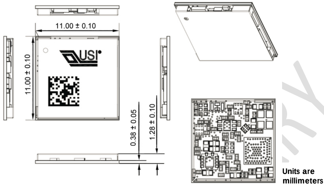
Figure 4: Mechanical Drawing
