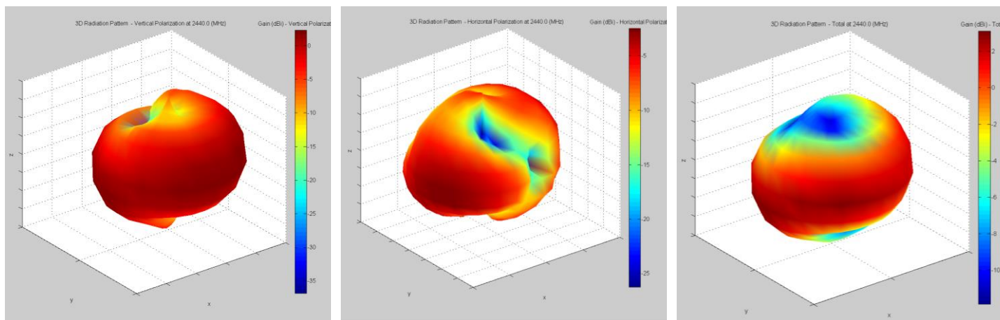
Figure 15: Vertical, horizontal, and total gain plots – 2440 MHz
