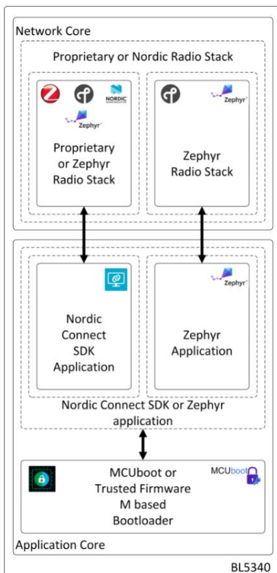
Figure 2: Functional SW block diagram for BL5340 series BLE module
