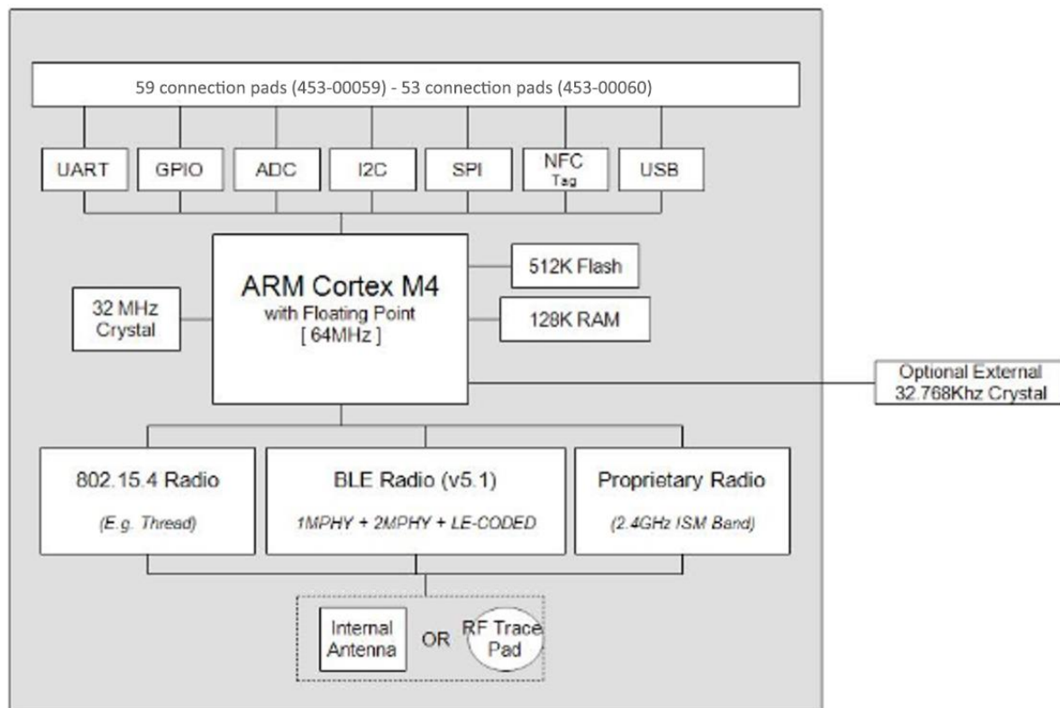
Figure 1: BL653μ block diagram
