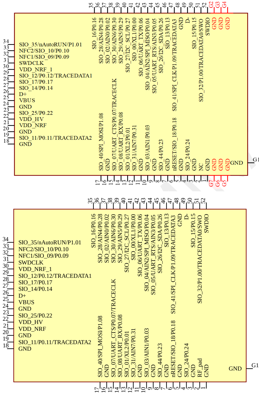
Figure 3: BL653μ module pin-out (top view).
