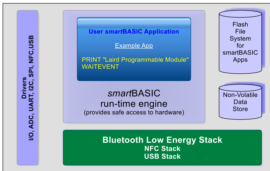
Figure 2: Functional HW and SW block diagram for BL653μ series BLE module
