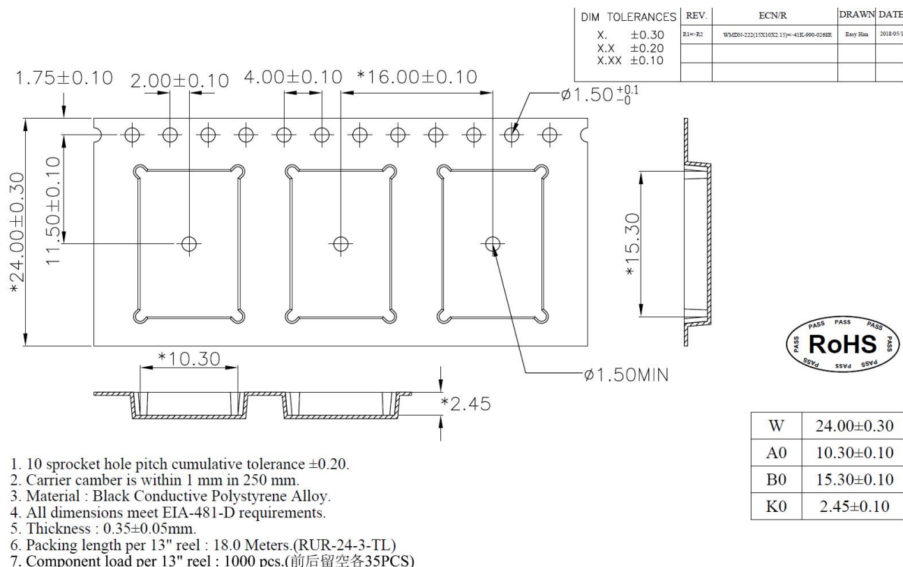
Figure 14: Tape specifications
