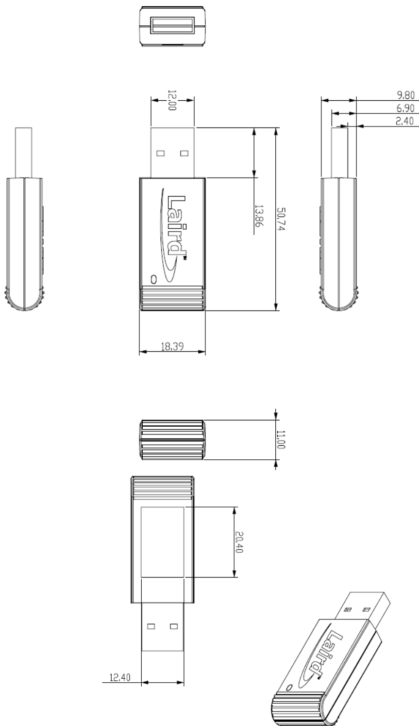
Figure 9: 451-00003 USB BLE 5.1 Dongle Mechanical details
