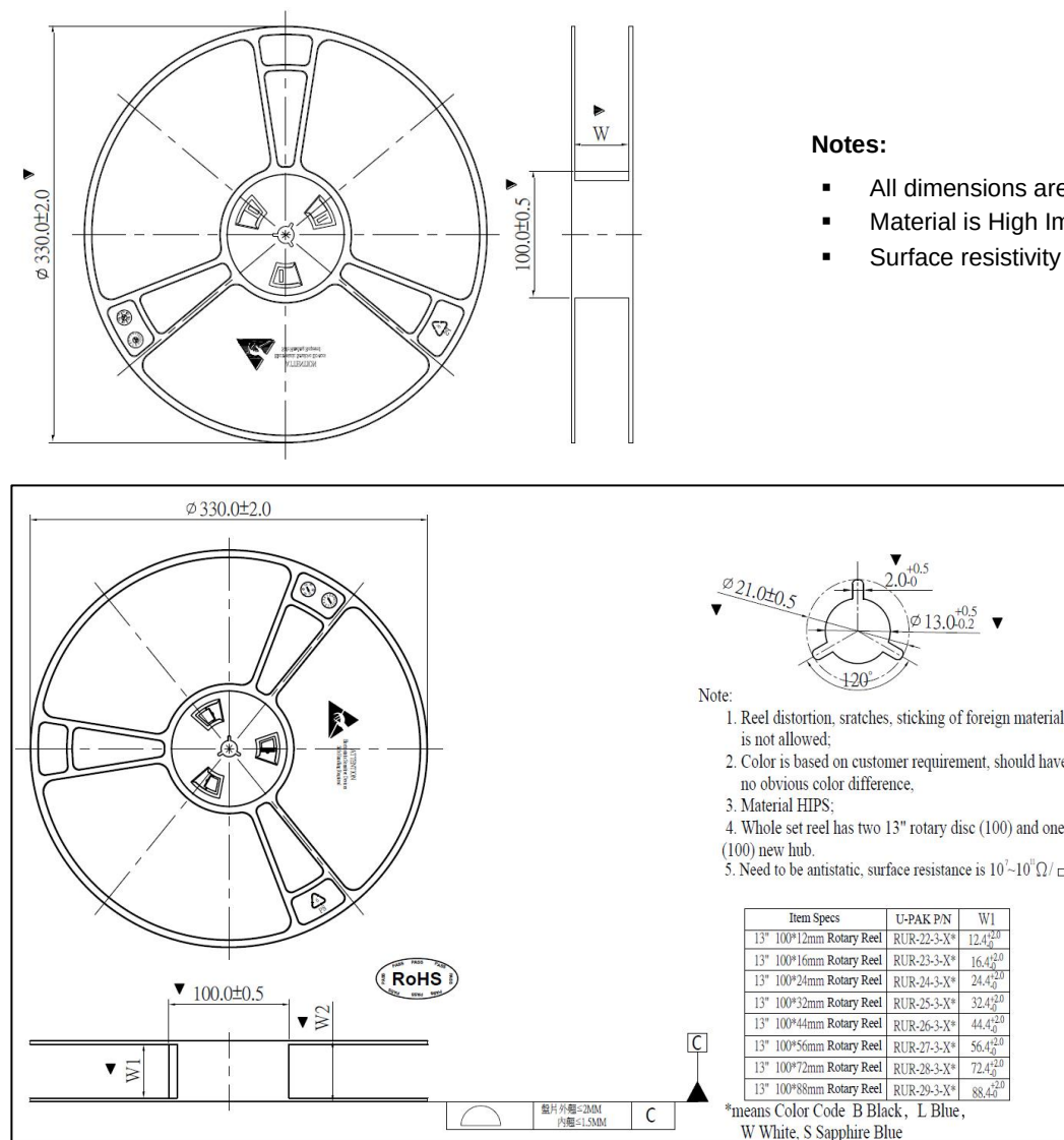
Figure 13: Reel specifications
