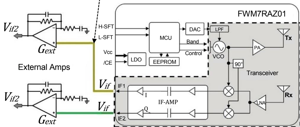
Fig. 5 Connection of external amplifier (example)
