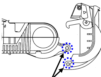
Opening and closing fulcrum of paper cover
