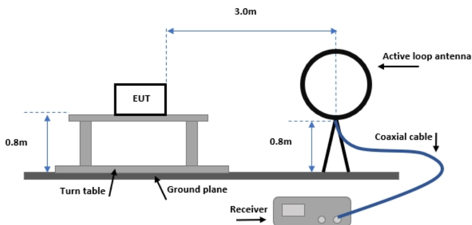
Radiated emissions test setup 9 kHz – 30 MHz
