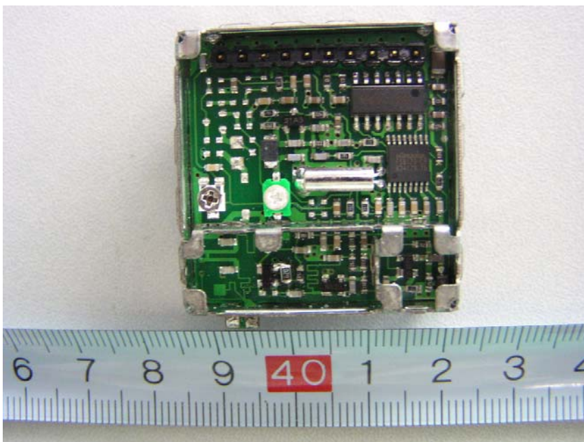
EUT – RF Module PCB Top View
