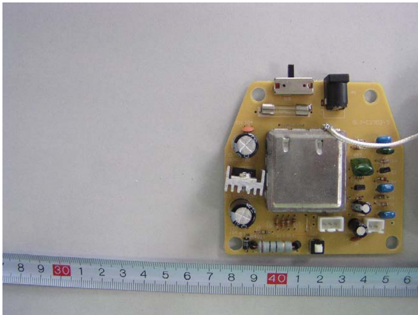
EUT – Main PCB Top View
