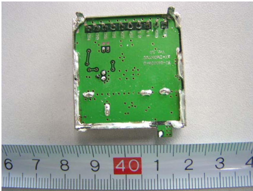
EUT – RF Module PCB Bottom View
