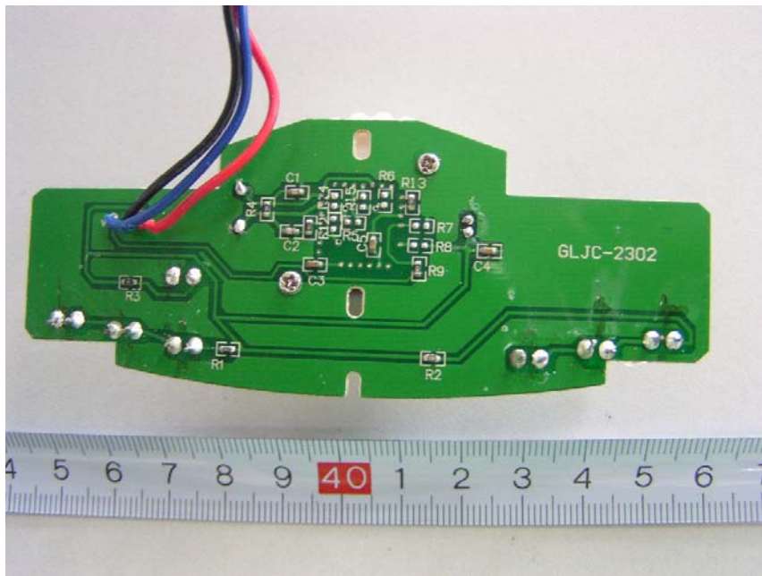
EUT – LED PCB Bottom View
