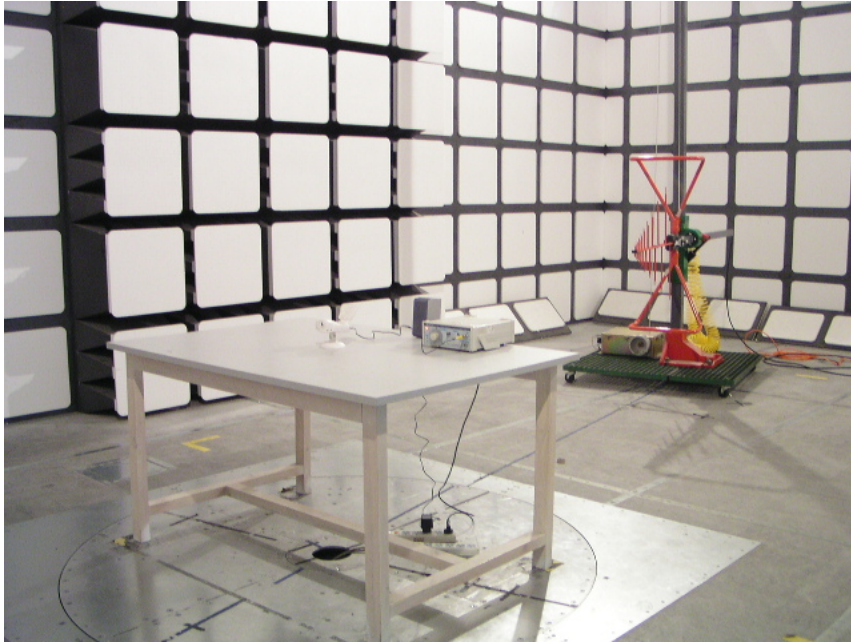
Radiated Emission - Front View (up to 1GHz)
