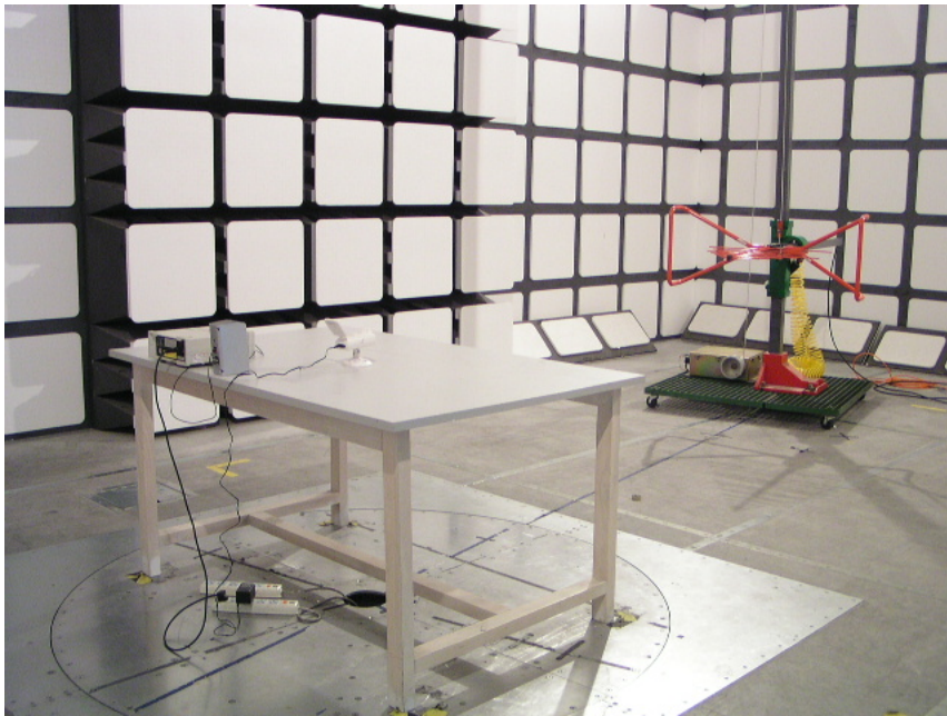
Radiated Emission - Rear View (up to 1GHz)
