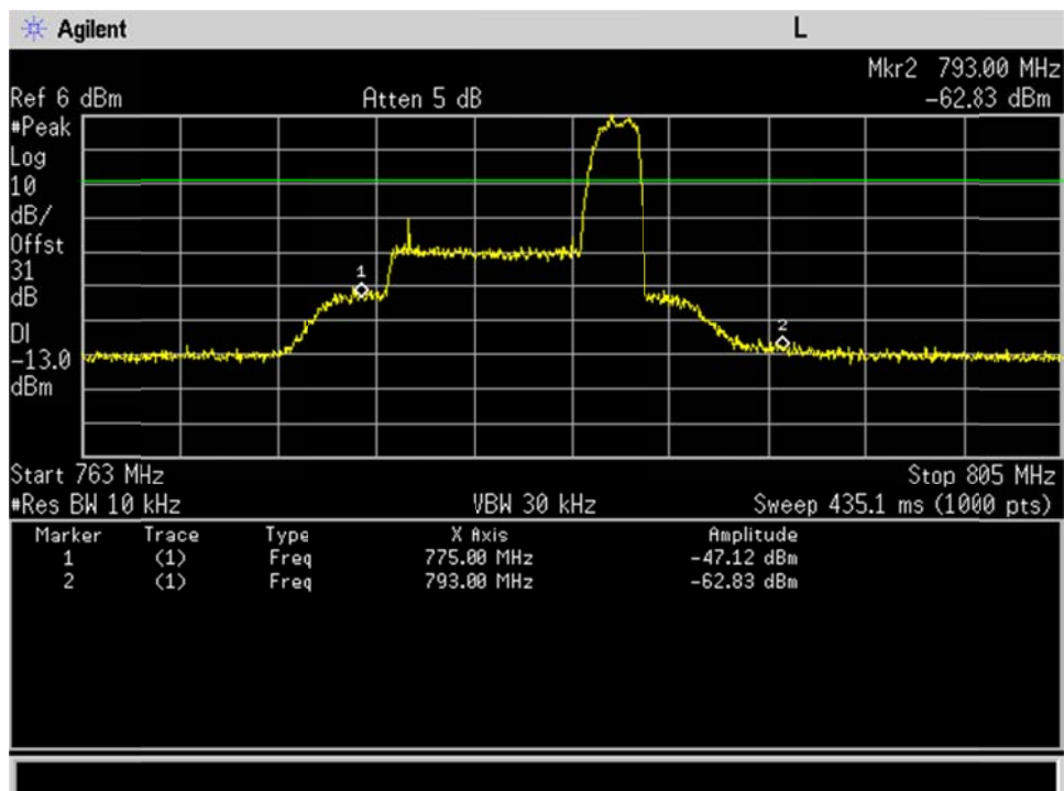
700 MHz uplink high_High Ch
