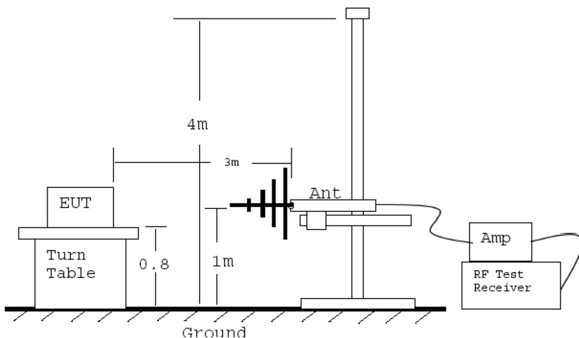
Radiated Emission Test 30 – 1000 MHz (Bilog)
