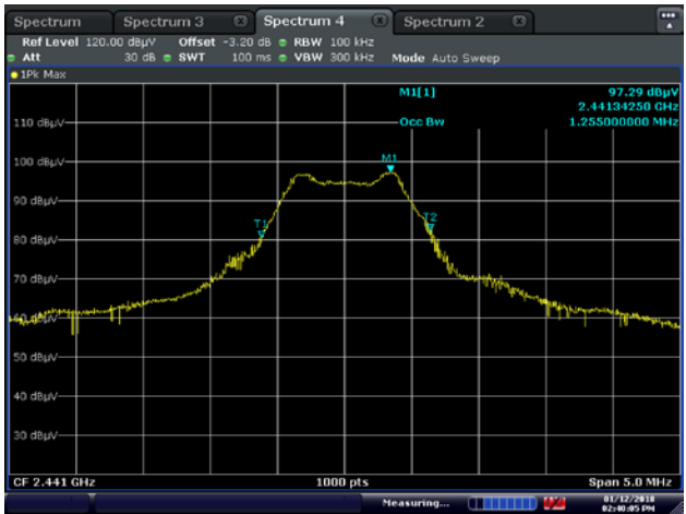
Figure 8.1-5: 99% OBW, Mid CH
