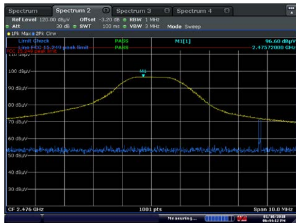
Figure 8.2-3: Fundamental emissions, High CH
