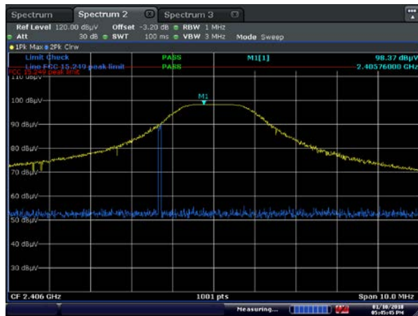
Figure 8.2-1: Fundamental emissions, Low CH
