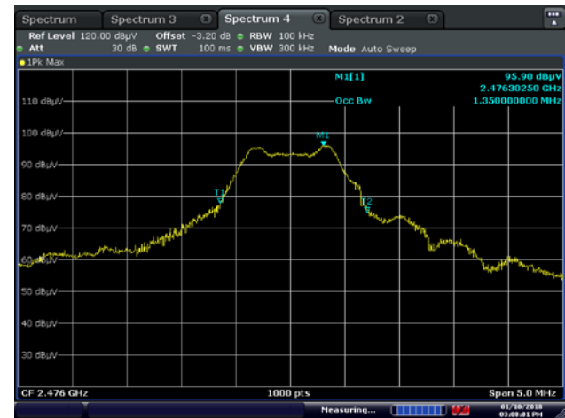
Figure 8.1-6: 99% OBW, High CH
