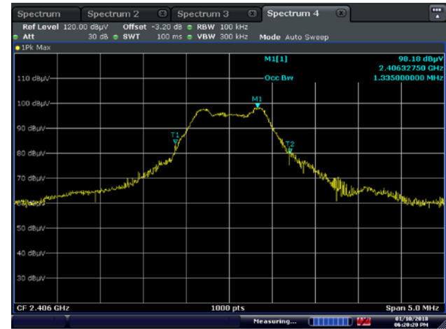
Figure 8.1-4: 99% OBW, Low CH
