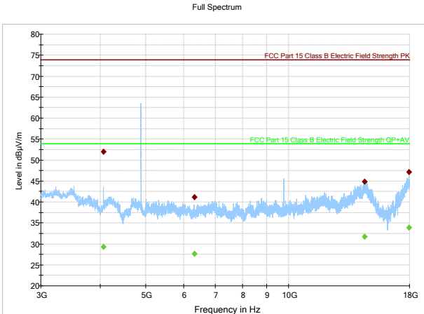
Figure 8.3-6: Radiated spurious emissions, Mid channel, 3-18GHz
