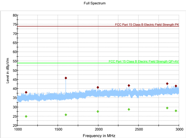
Figure 8.3-2: Radiated spurious emissions, low channel, 1-3GHz
