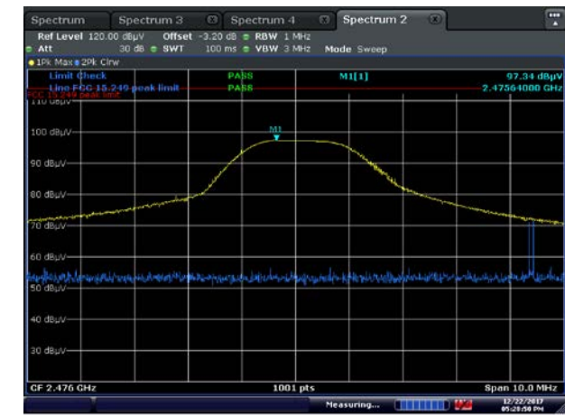
Figure 8.2-3: Fundamental emissions, High CH
