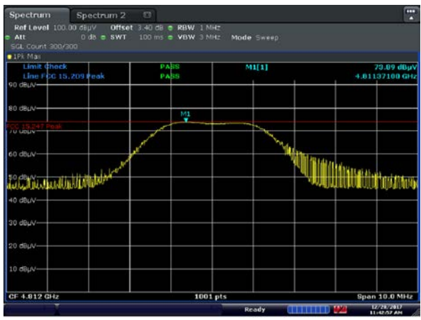
Figure 8.2-4: 2 nd harmonic emissions, Low CH
