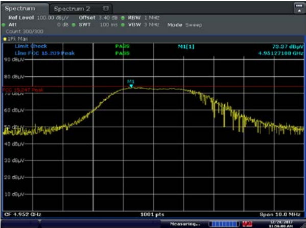
Figure 8.2-6: 2 nd harmonic emissions, High CH
