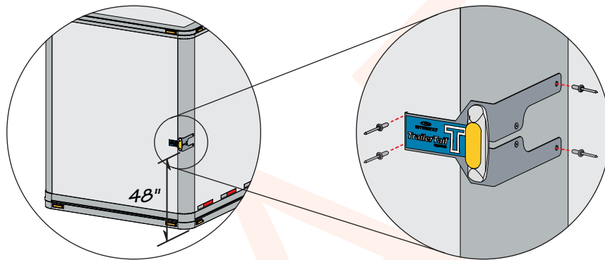
Secure the Warning Light
