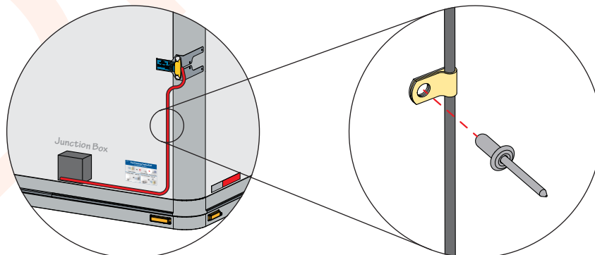
Riveted Wire Clamps
