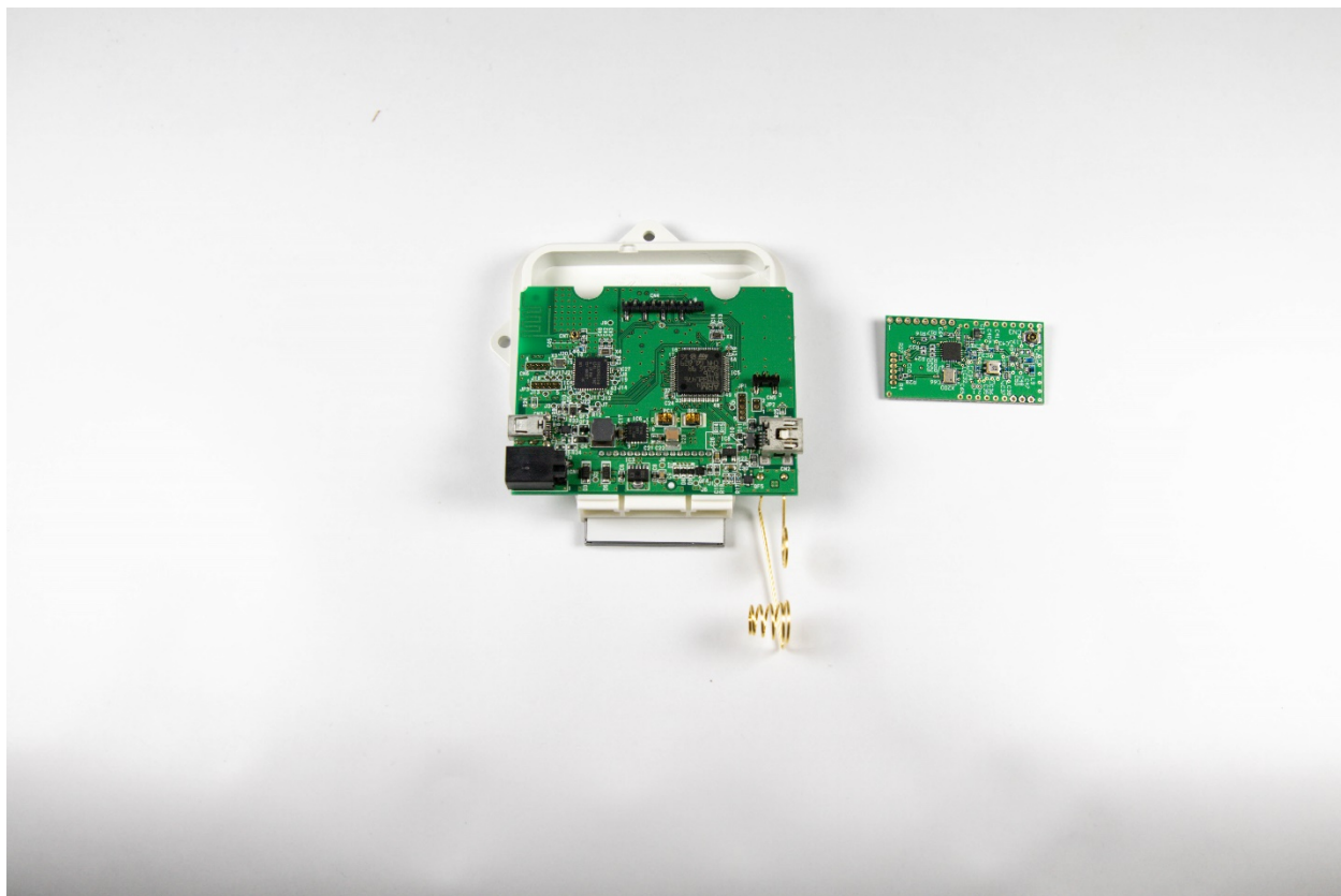
PCB with RF Board Removed
