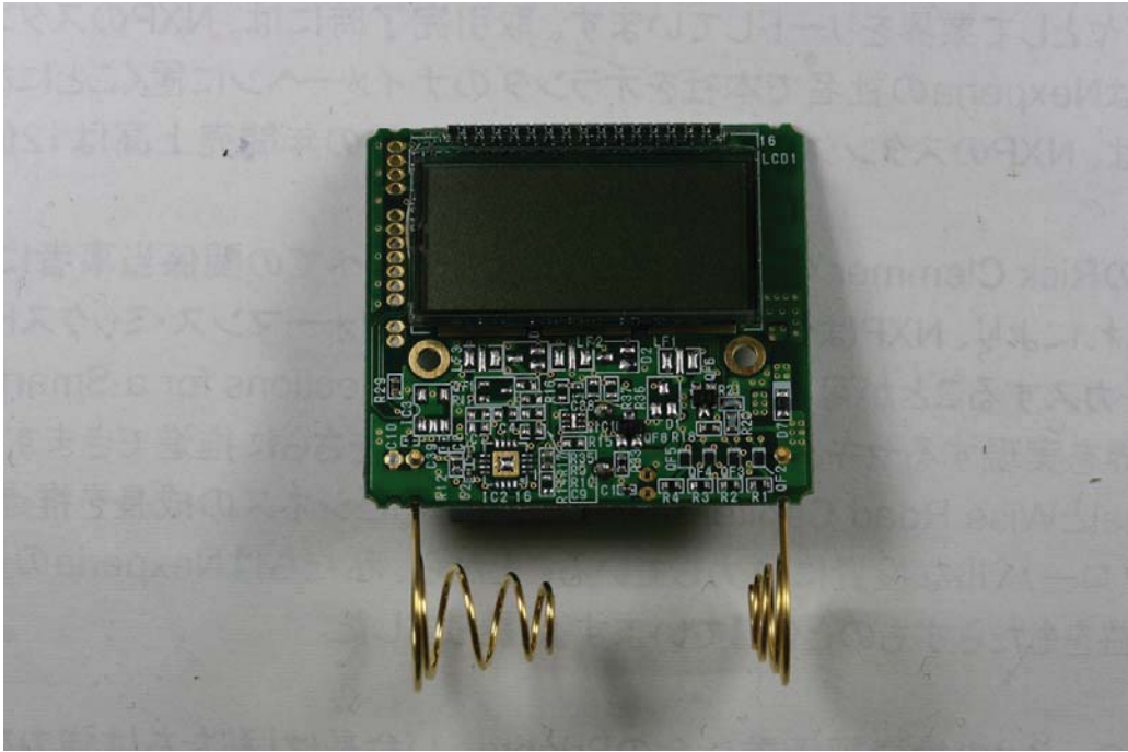
Cover Removed
