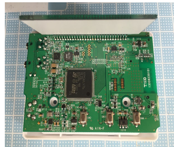
Board A side Inside of LCD
