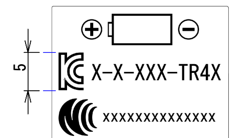
Certification Label Scale(2 : 1)
