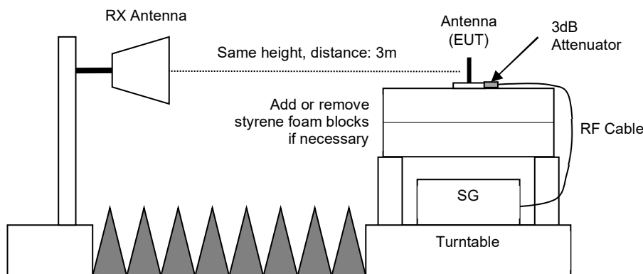
Figure 1: Block Diagram
