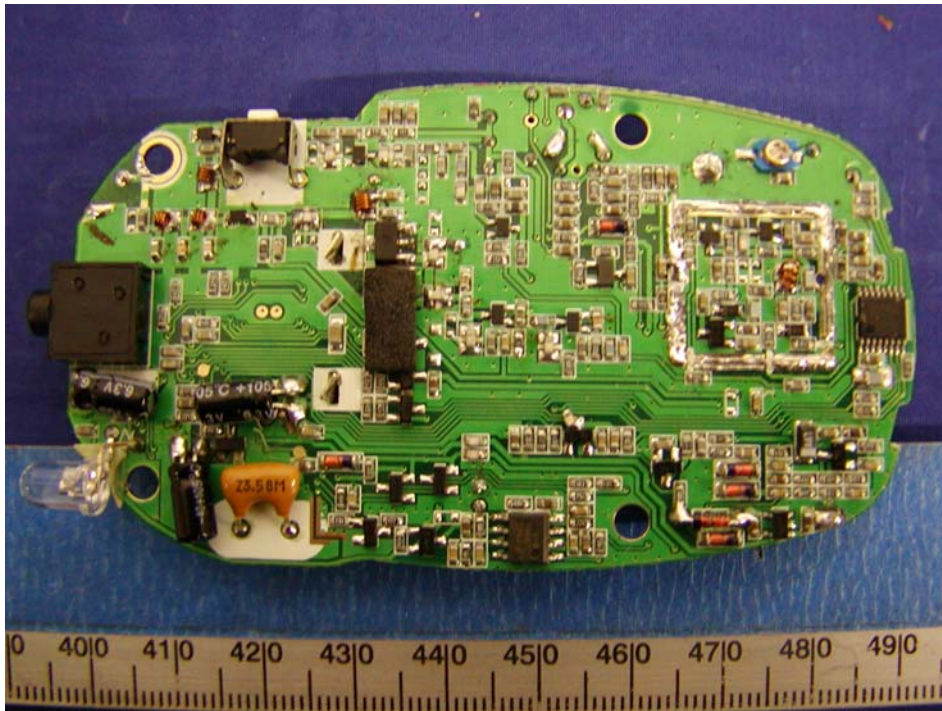
EUT – Component View without Shielding
